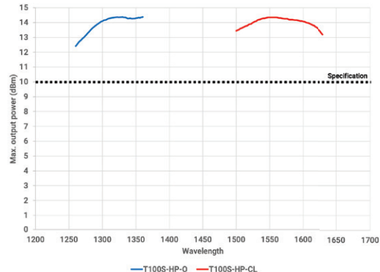
Figure 1. Typical maximum optical output power for the essential models
